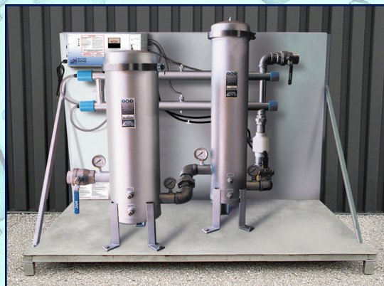
Custom Engineered Multi-Process Modular Water Treatment System, Designed to Customer' Specifications.
